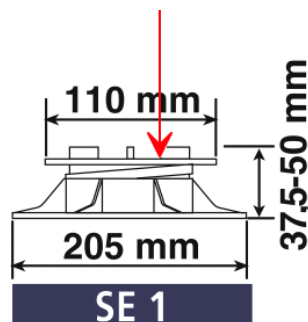
Figure 2 Typical "ETERNO SE1" specimen.
