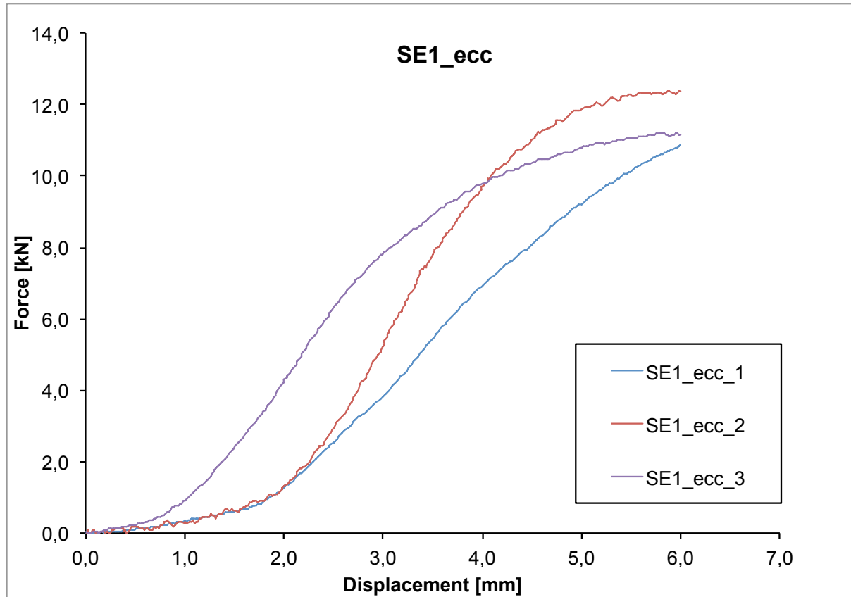
Figure 1 Diagram force versus displacement of testing machine's crossbar for "ETERNO SE1" specimen.
