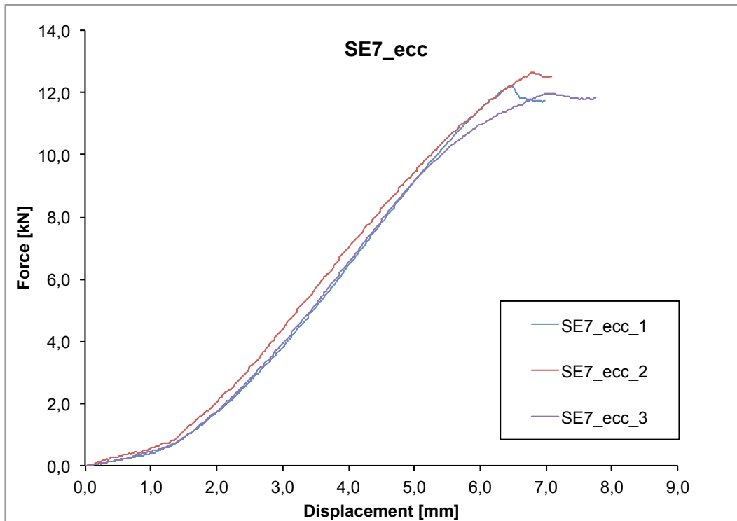
Figure 1 Diagram force versus displacement of testing machine's crossbar for "ETERNO SE7" specimen.
