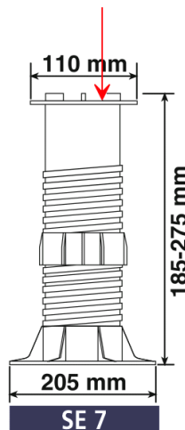
Figure 2 Typical "ETERNO SE7" specimen.
