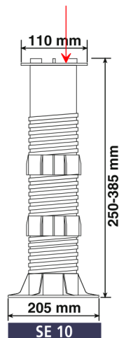
Figure 2 Typical "ETERNO SE10" specimen.
