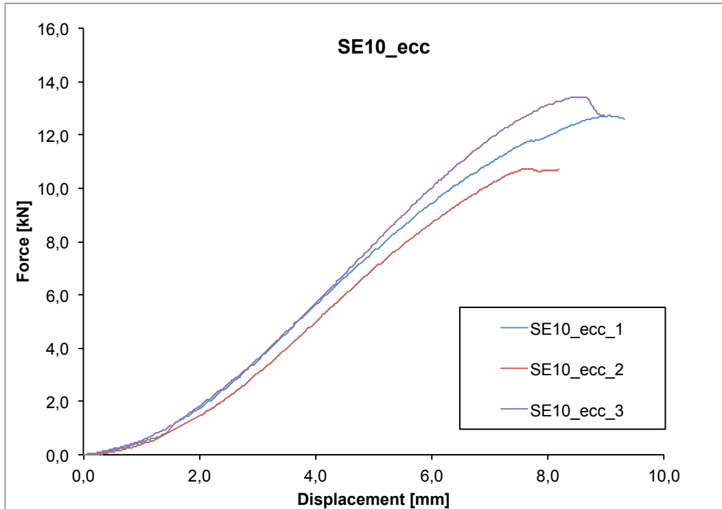
Figure 1 Diagram force versus displacement of testing machine's crossbar for "ETERNO SE10" specimen.
