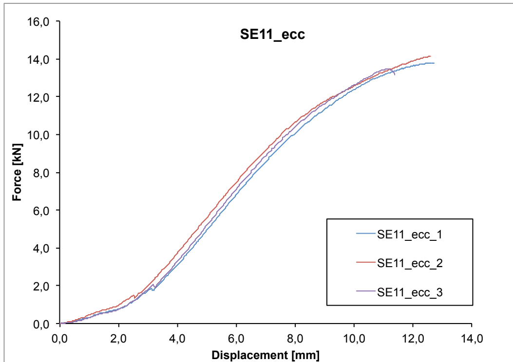
Figure 1 Diagram force versus displacement of testing machine's crossbar for "ETERNO SE11" specimen.
