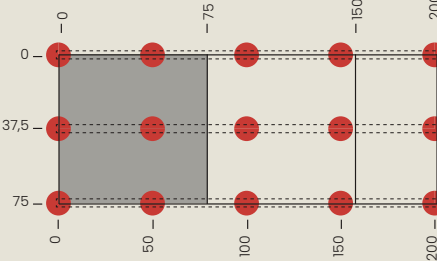
Lastra | Slab 80 x 80 cm - Interasse travetto | Interaxle joist 40 cm
