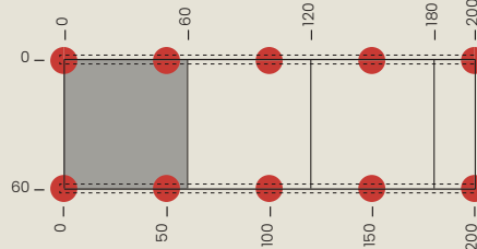
Lastra | Slab 60 x 60 cm - Interasse travetto | Interaxle joist 60 cm
