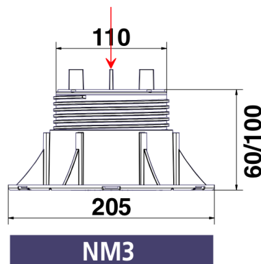
Figure 2 Typical "New-Maxi NM3" specimen.
