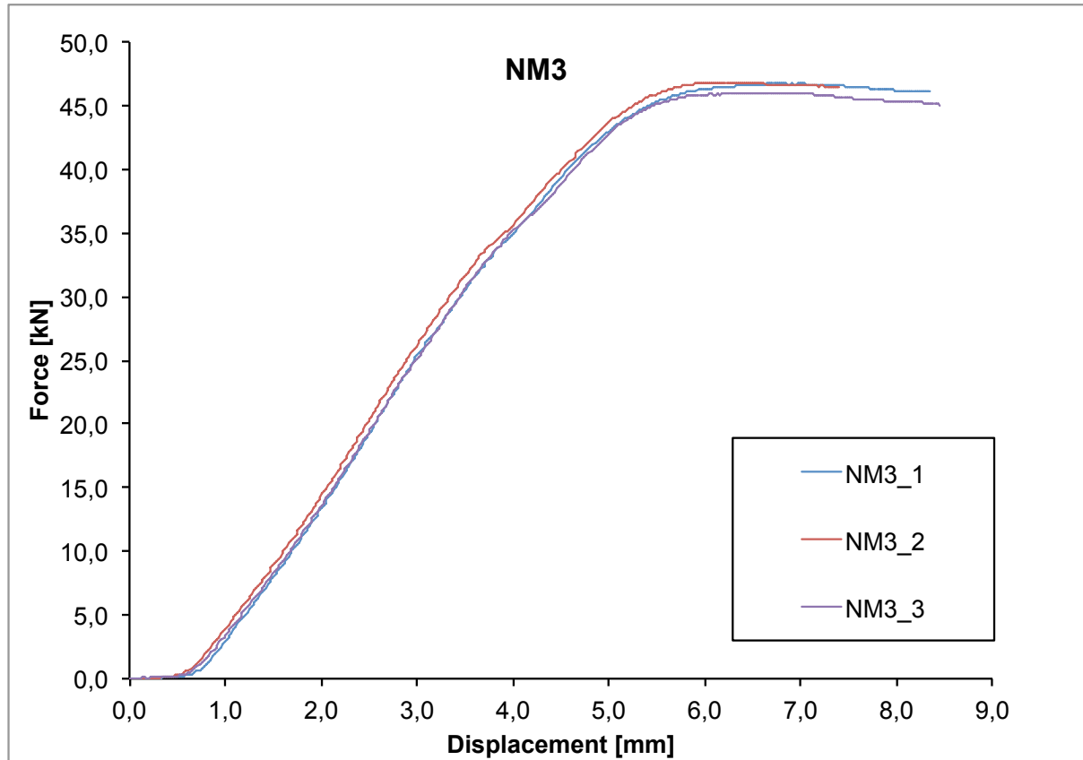
Figure 1 Diagram force versus displacement of testing machine's crossbar for "NEW-MAXI NM3" specimen.
