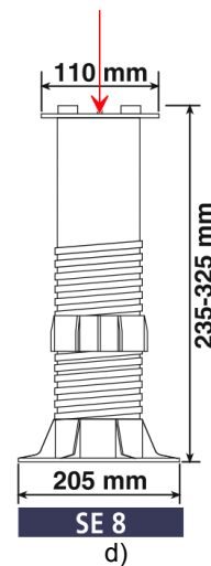
Figure 1 Diagram force versus displacement of testing machine's crossbar for Hmax (a), Hmed (b), Hmin (c) and typical "Eterno SE8" specimen (d).
